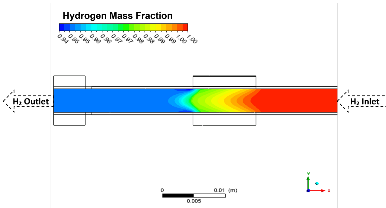
Figure 4.14: Hydrogen mass fraction across the tubular cell at the operating conditions shown in Table 4.3.
