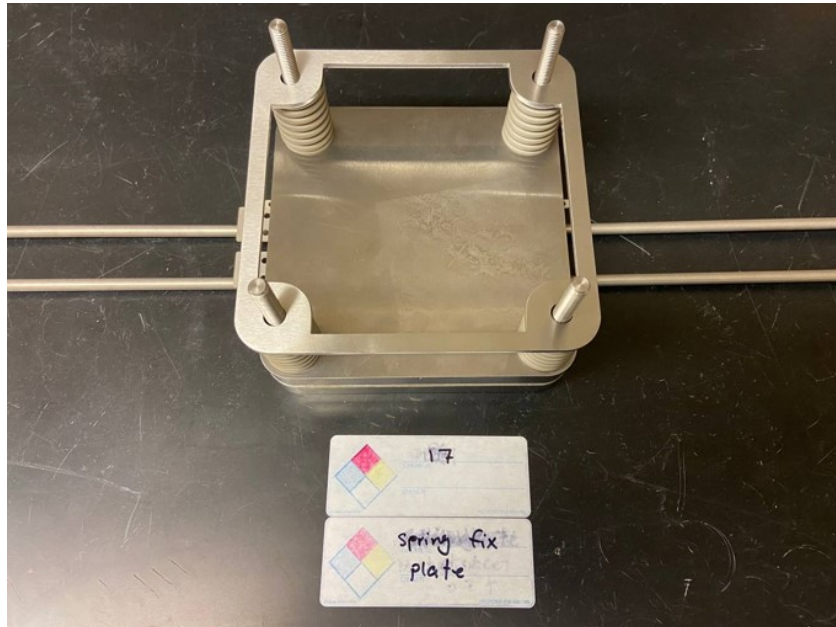
Figure A.15: Planar SOFC stack assembly step 17
