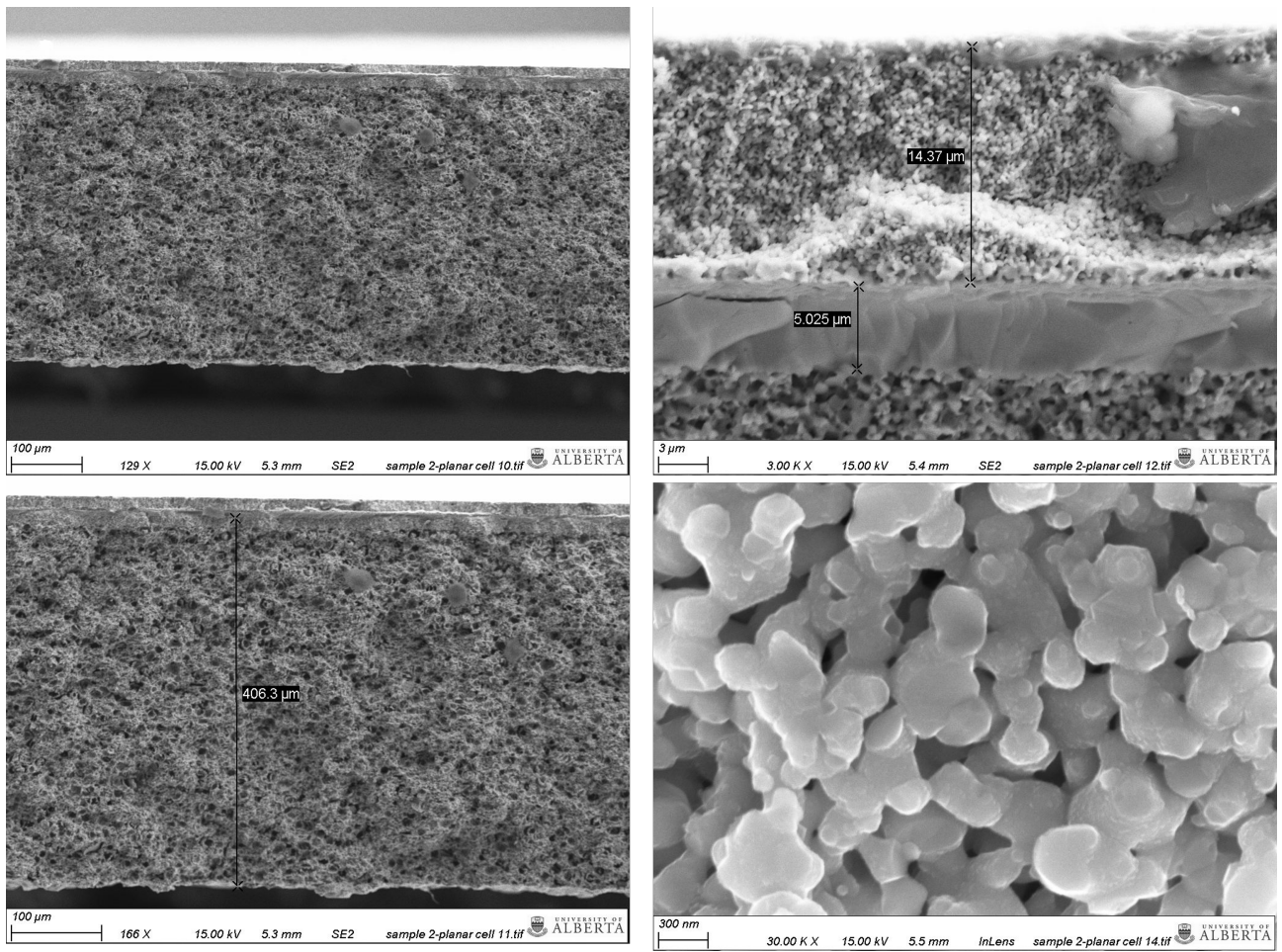
Figure C.2: Planar cell SEM images.
