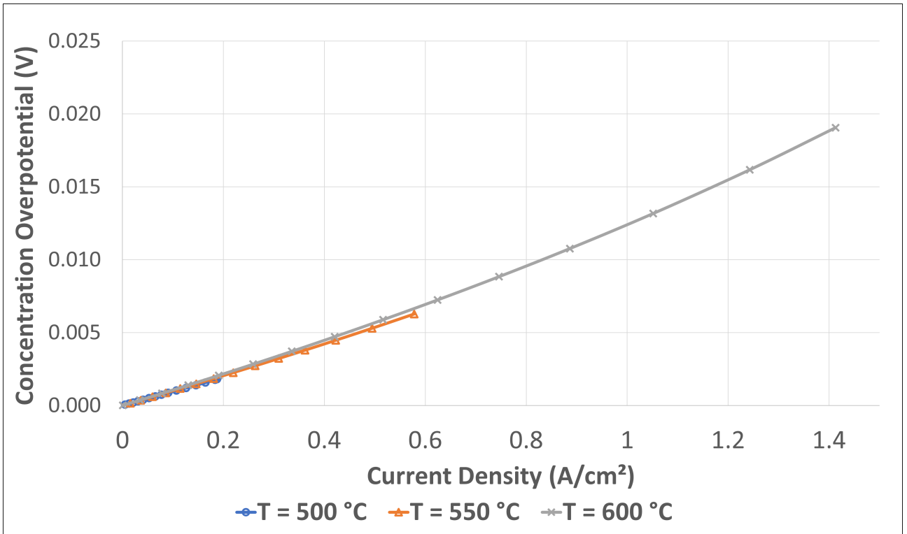
Figure 4.5: The effect of cell's operating temperature on the concentration overpotential of the tubular cell.
