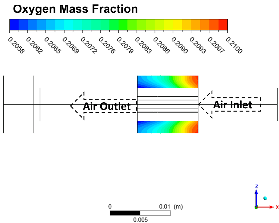
Figure 4.15: Oxygen mass fraction across the tubular cell at the operating conditions shown in Table 4.3.
